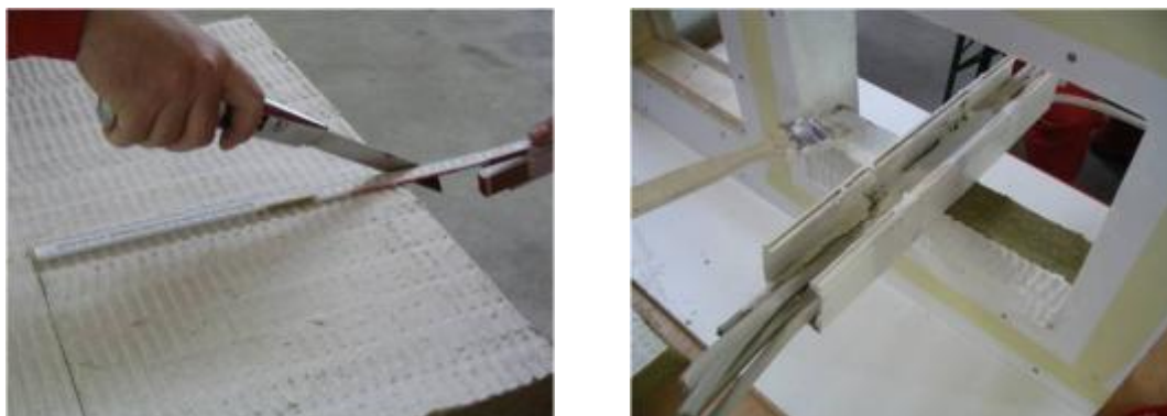
Figure 85: Cut to size of mineral fiberboard and coating of boards and reveal, source: Würth company
