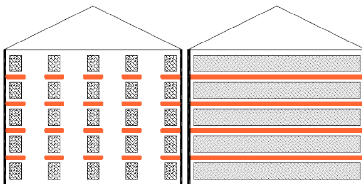
Figure 103: Example of the arrangements of fire protection partitions with perforated facades or strips of ribbon windows
