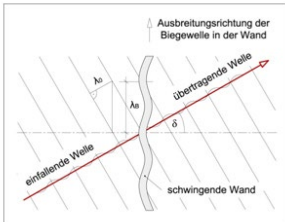
Figure 19: Coincidence
