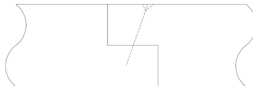
Figure 59: Remaining wood cross section in the joint area of rebated connections
