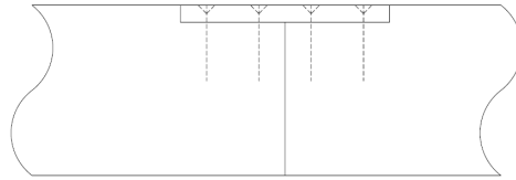
Figure 58: Remaining wood cross section in the joint area of melted boards
