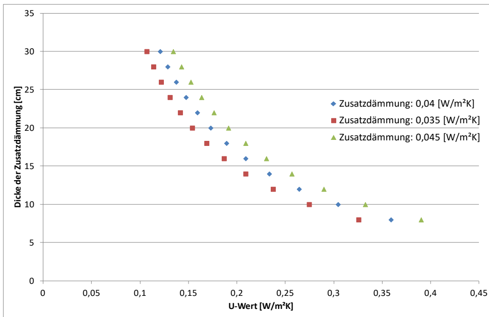
Figure 28: U values of a 8cm thick cross-laminated timber wall ( \lambda : 0.13 W/m 2 K) as a function of thickness and heat conductivity of additional insulation
