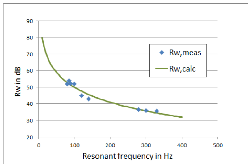
The Figure shows a comparison of measured and calculated weighted sound reduction index R_w of CLT with ETICS
